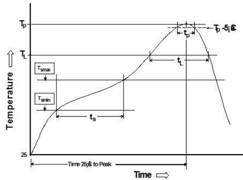
Tin/Lead Recommended Reflow Profile (Based on J-STD-020D)
