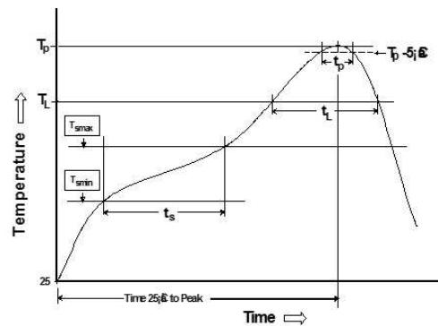
No Lead Recommended Reflow Profile (Based on J-STD-020D)
